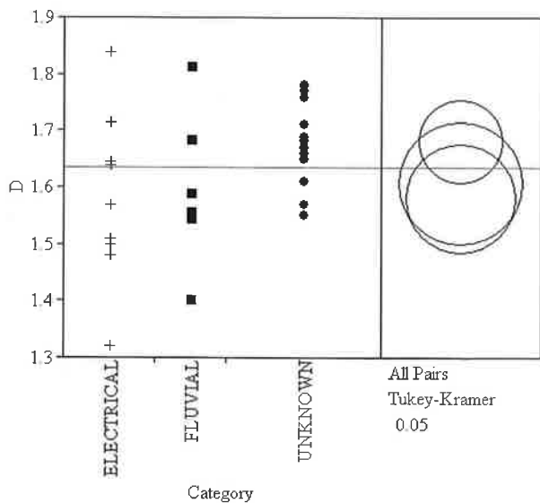
Fig. 2. Tukey-Kramer comparisons of various measured D -values of three categories of measurements. Overlapping circles denote no statistical difference based on a 95% confidence interval.
