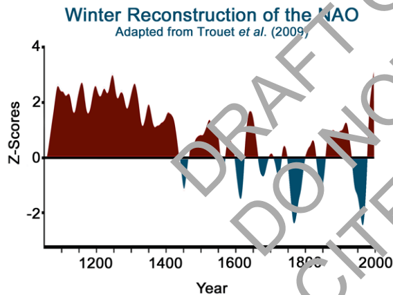
Figure 4.2.4.6.3.3. Winter reconstruction of the NAO over the past 1,000 years. Adapted from Trouet et al. (2009).
