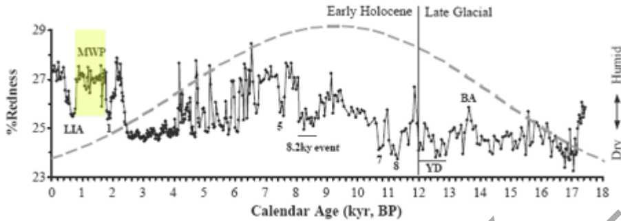
Figure 4.2.4.1.3. Qinghai Lake climate proxy showing the presence of the Little Ice Age and Medieval Warm Period as determined by the % redness value in a lake sediment core. Adapted from Ji et al. (2005).
