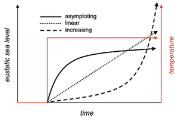
Figure 6.2.1.1.3. Three alternative models for sea-level rise. Adapted from PALSEA, 2009. The sea-level conundrum: case studies from palaeo-archives: Journal of Quaternary Science 25 : 19–25; PALSEA, 2012. Sea level and ice sheet evolution. De Menocal, P. (Ed.) Earth and Planetary Science Letters, Special Edition 315–316 : 1–102.
