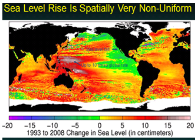
Figure 6.2.1.3.2. Synoptic global map of rate of sea-level change 1993-2008, as measured by radar altimetry. Adapted from NOAA 2007. http://www.oco.noaa.gov/resources/Annual_Program_Reports/FY07_Program_Report/chapterII/09-1-Miller_FY07_Altimetry.pdf .
