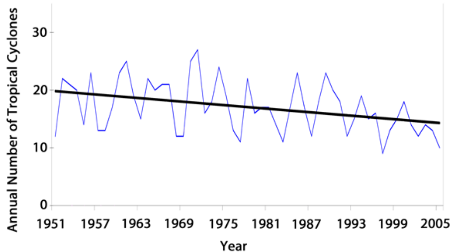
Figure 7.10.3.3. Number of typhoons affecting China (1951-2005). Adapted from Sun, L.-h., Ai, W.-x., Song, W.-l. and Wang, Y.-m. 2011. Study on climatic characteristics of China-influencing tropical cyclones. Journal of Tropical Meteorology 17: 181-186.
