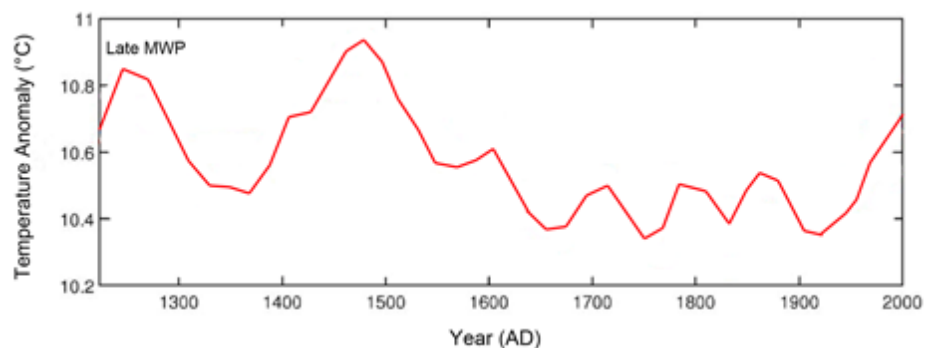
Figure 4.2.4.6.2.1. Decadally smoothed diatom-based temperature reconstruction from Lake Tsuolbmajavri in Finnish Lapland. Adapted from Weckstrom et al. (2006).
