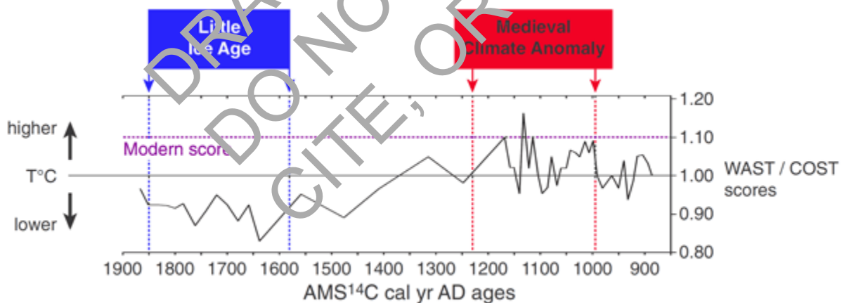
Figure 4.2.4.4.1. The 880-1870 cal yr AD warm-cool ratio WAST/COST temperature reconstruction of Kaniewski et al. (2011). Adapted from their Figure 5.
