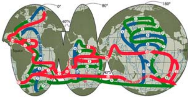
Figure 6.2.3.2.2. Schmitz (1996) summary of the main components of global ocean circulation. The volume transport rates in Sverdrups ( 1 \text{ Sv} = 106 \text{ m}^3 \cdot \text{s}^{-1} ) are indicated in the circles. Adapted from Schmitz, W.J. 1996. On the World Ocean Circulation: Volume II—The Pacific and Indian Oceans / A Global Update . Technical Report, Woods Hole Oceanographic Institution, p. 245.
