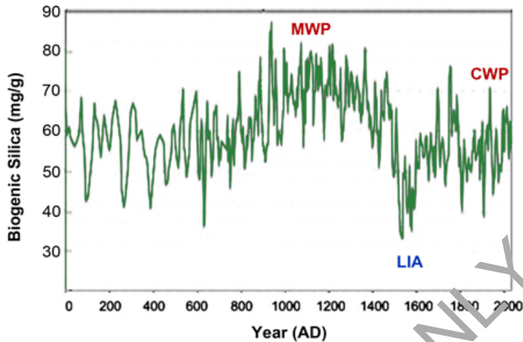
Figure 4.2.4.6.3.4. A 2,000-year record of climate variations reconstructed from Haukadalsvatn, West Iceland. Adapted from Geirsdottir et al. (2009).
