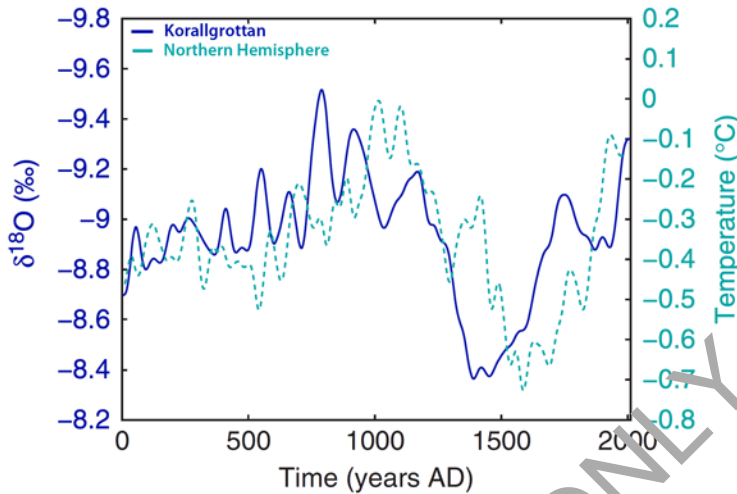
Figure 4.2.4.6.2.9. The 2,000-year Northern Hemisphere temperature reconstruction (dashed line) of Moberg et al. (2005) and the last half of the \delta^{18}\text{O} history (solid line) developed from the K11 stalagmite. Adapted from Sundqvist et al. (2010).
