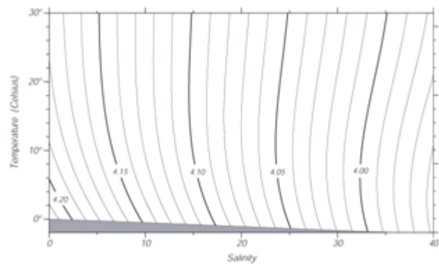
Figure 6.2.2.1.1. Specific heat of seawater in \text{J}\cdot\text{g}^{-1}\cdot\text{C}^{-1} at atmospheric pressure for a typical range of ocean temperatures and salinities http://oceanworld.tamu.edu/resources/ocng_textbook/chapter05/chapter05_01.htm .
