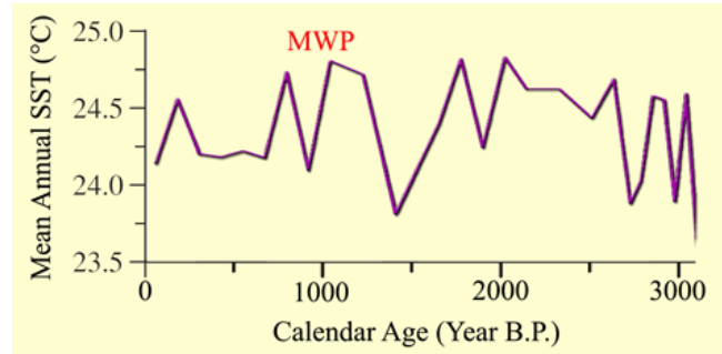
Figure 4.2.4.8.2.3. Sea surface temperature proxy derived from a gravity core recovered from the East China Sea. Adapted from Fengming et al. (2008).
