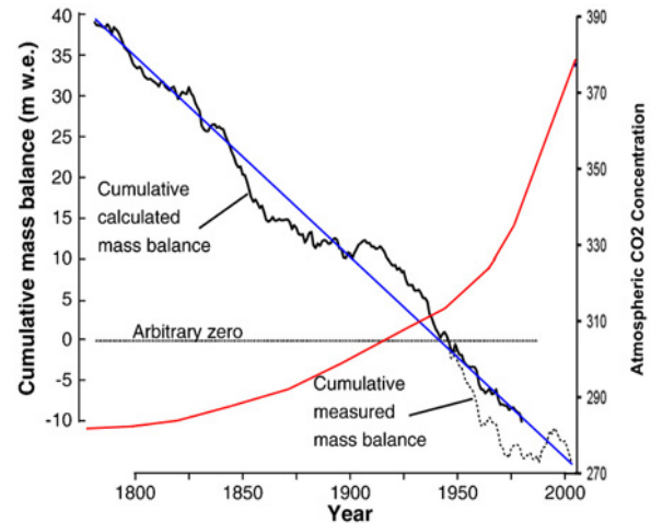
Figure 5.9.2.2. The cumulative reconstructed net mass balance history of Sweden's Storglaciaren, to which we have added the fit-by-eye descending linear relationship (blue line), and the history of the atmosphere's CO 2 concentration (red line). Adapted from Linderholm, H.W., Jansson, P., and Chen, D. 2007. A high-resolution reconstruction of Storglaciaren mass balance back to 1780/81 using tree-ring and circulation indices. Quaternary Research 67 : 12–20.
