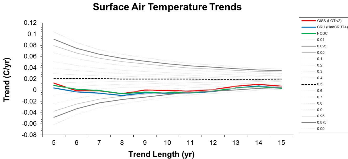
Figure 1.3.6.1.3. Trends (through 2012) in three observed global surface temperature records of length 5 to 15 years (colored lines) set against the probability (gray lines) derived from the complete collection of climate model runs used in the IPCC Fourth Assessment Report under the SRES A1B emissions scenario. Reprinted with permission from Knappenberger, P.C. and Michaels, P.J., 2013. Policy implications of climate models on the verge of failure. American Geophysical Union Science Policy Conference. Washington, DC, June 24–26, 2013.
