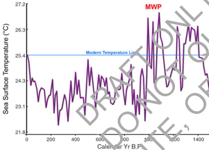
Figure 4.2.4.7.2.3. Annual Mg/Ca-derived SST anomalies for Pigmy Basin, Northern Gulf of Mexico. Adapted from Richey et al. (2007).
