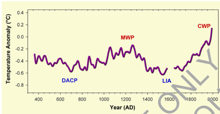
Figure 4.2.4.9.6.1. Reconstructed tropical South American temperature anomalies normalized to the AD 1961–1990 average and smoothed with a 39-year Gaussian filter. Adapted from Keilerhals et al. (2010).
