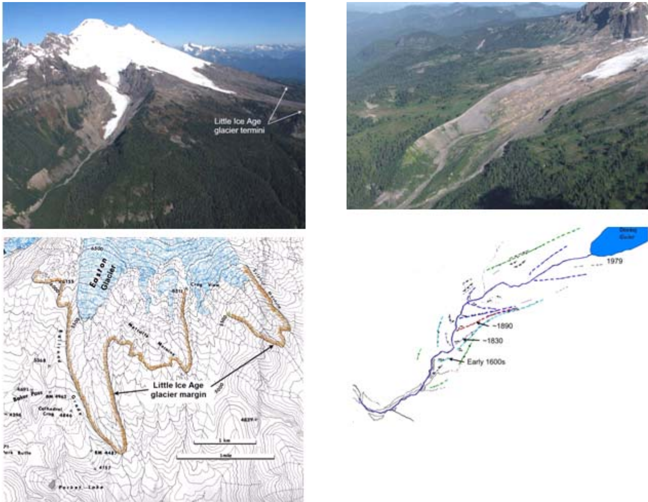
Figure 5.9.6.1. LEFT COLUMN: Photo (upper) and topographic map (lower) of ice retreat from the Little Ice Age maximum, Deming and Easton glaciers, Mt. Baker Washington. RIGHT COLUMN: Photo (upper) and sketch map (lower) of dated moraines down-valley from the Deming glacier on Mt. Baker, Washington. All adapted from Easterbrook, D.J. 2011. Geologic evidence of recurring climate cycles and their implications for the cause of global climate changes—the past is the key to the future. Elsevier, pp. 3–51.
