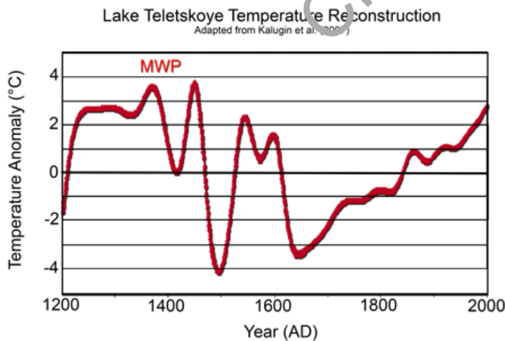
Figure 4.2.4.4.3.2. Proxy temperature record of Lake Teletskoye in the Altai Mountains in southern Siberia. Adapted from Kalugin et al. (2007).
