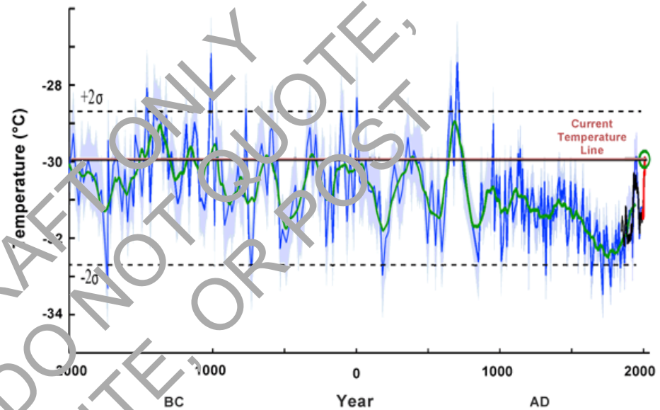
Reconstructed Greenland Temperature Over the Past 4000 Years
