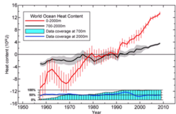
Figure 6.2.2.2.1. Smoothed (pentadal) ocean heat estimates for 0–2000 m and 700–2000 m. The average temperature increases associated with the changed heat contents are 0.09°C and 0.18°C for the top 2000 m and 700 m respectively. Adapted from Levitus, S., Antonov, J.I., Boyer, T.P., Baranova, O.K., Garcia, H.E., Locarnini, R.A., Mishonov, A.V., Reagan, J.R., Seidov, D., Yarosh, E.S., and Zweng, M.M. 2012. World ocean heat content and thermosteric sea level change (0–2000 m), 1955–2010: Geophysical Research Letters 39 : L10603–L10603.
