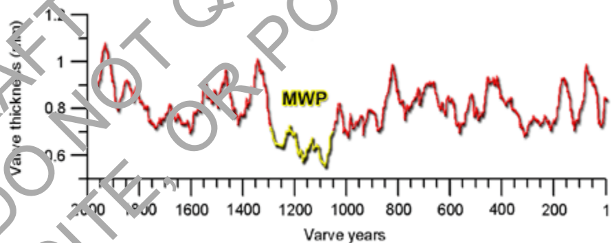
Figure 4.2.4.6.2.2. Varve thickness from sediment cores obtained from Lake Lehmilampi, eastern Finland. Adapted from Haltia-Hovi et al. (2007).
