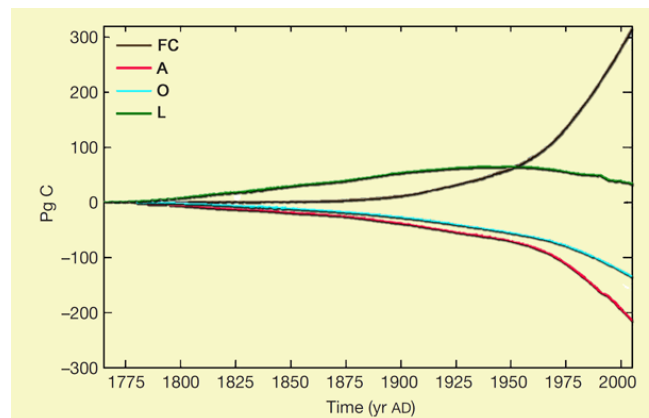
Figure 2.6.1.2. The evolution of anthropogenic-produced carbon originating from fossil fuel use and cement production (FC), together with the similar evolution of the three anthropogenic carbon sinks—atmosphere (A), ocean (O), and land (L)—between AD 1765 and 2005. Adapted from Khatiwala, S. Primeau, F., and Hall, T. 2009. Reconstruction of the history of anthropogenic CO 2 concentrations in the ocean. Nature 462 : 346–349.
