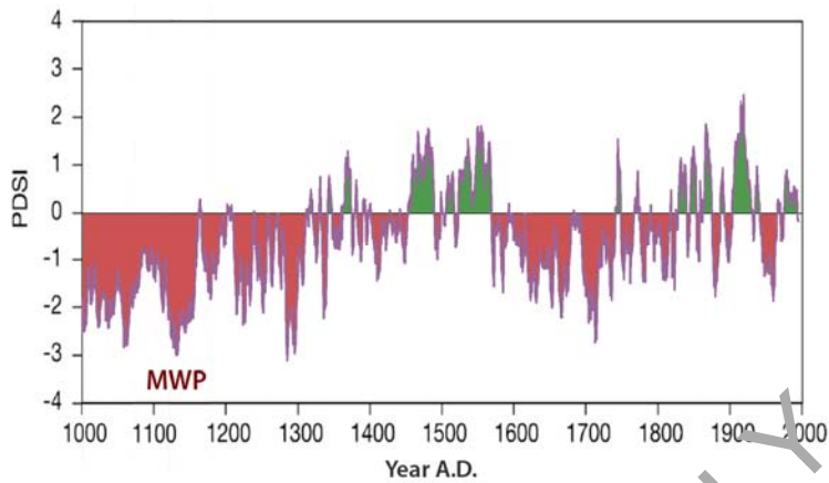
Figure 4.2.4.7.2.4. Reconstructed winter PSDI for Southern California since AD 1100. Adapted from MacDonald et al. (2008).
