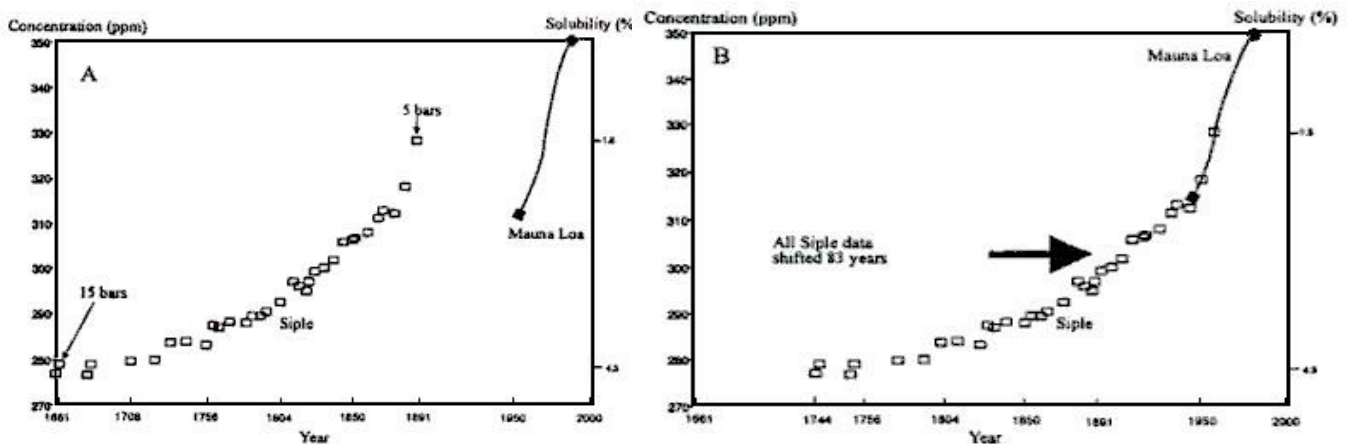
Figure 1 Concentration of CO 2 in air bubbles from the pre-industrial ice from Siple, Antarctica (open squares), and in the 1958-1986 atmosphere at Mauna Loa, Hawaii (solid line): (A) original Siple data without assuming a 83 year younger age of air than the age of the enclosing ice, and (B) the same data after arbitrary "correction" of age of air (Neftel et al., 1985; Friedli et al., 1986; and IPCC, 1990).
