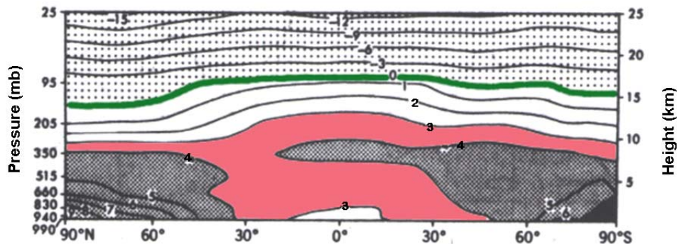
Figure 11. Same as Figure 10 but for the NOAA-GFDL GCM.
