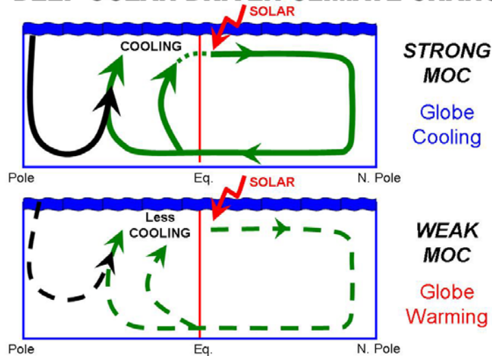
Figure 17. Idealized North-South graphical illustration of a strong (top) and weak (bottom) MOC. It is hypothesized that these differences in MOC strength are caused by salinity variations.
