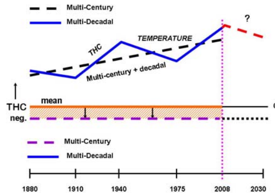
Figure 28. Idealized portrayal of how a combination of weak and strong multi-decadal variations in THC in combination with a century-scale long weak THC (or MOC) could well explain the long term up-and-down trend in global temperature over the last 130 years.
