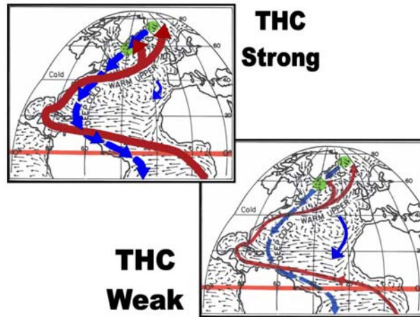
Figure 25. Portrayal of strong and weak THC conditions.
