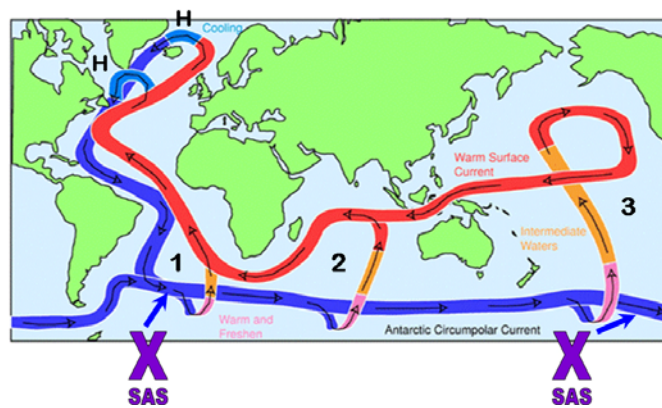
Figure 14. Idealized portrayal of the deep water Global Ocean Conveyor Belt (often referred to as the MOC) showing the typical locations in the Southern Hemisphere where upwelling occurs into the upper ocean thermocline and mixed layer (areas 1, 2, and 3) that is required to balance THC subsidence (H areas). Surrounding Antarctic Subsidence (SAS) is shown by X's. The MOC = (THC + SAS). Estimates are that the mass of the North Atlantic deep water subsidence is about twice the mass as the ocean subsidence around Antarctica. Over multi-decadal periods THC and SAS are positively related to each other. Figure adapted from John Marshall, of MIT.
