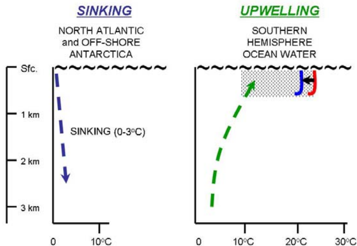
Figure 16. Illustration of how cold water subsidence in polar regions and compensating upwelling in the Southern Hemisphere tropics could lead to upper ocean cooling.
