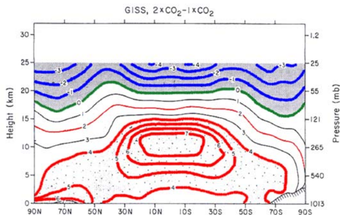
Figure 10. North-South vertical-cross section showing Hansen's early GCM's model change in temperature ( ^{\circ}\text{C} ) that would accompany a doubling of atmospheric \text{CO}_2 . There is no way a doubling of \text{CO}_2 and an extra 3.7 \text{ W/m}^2 blockage of OLR to space could lead to such extreme upper tropospheric temperature rises. These large temperature increases occurred because of Hansen's unrealistic upper level water vapor assumptions.
