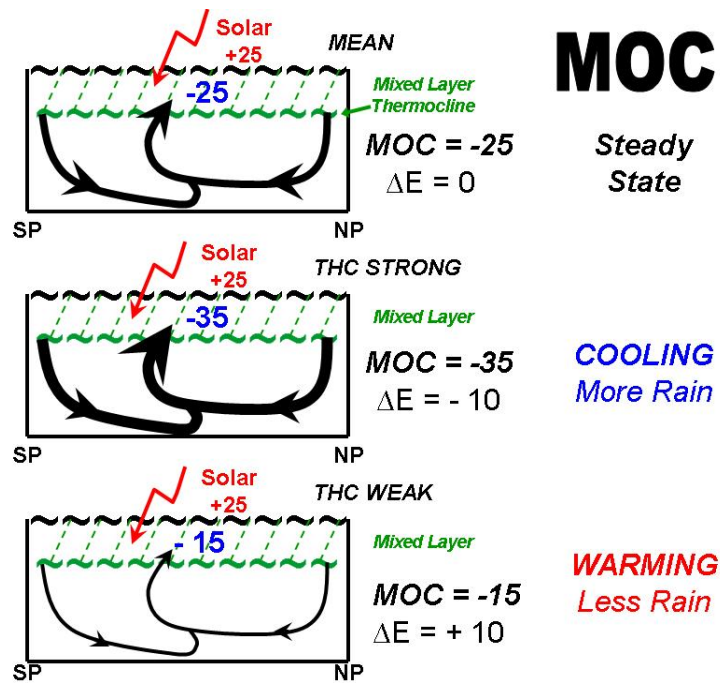
Figure 18. Hypothesized global MOC induced upper ocean energy budget for steady (top), cooling (middle) and warming (bottom) global conditions. Observations indicate that the globe has somewhat more rainfall when the MOC is strong than when it is weak. MOC units in Sverdrups ( 10^{12} gm/s). \Delta E gives upper ocean energy changes. There is theoretical and observational evidence that north and south polar subsidence is related to each other over longer multi-decadal time periods.
