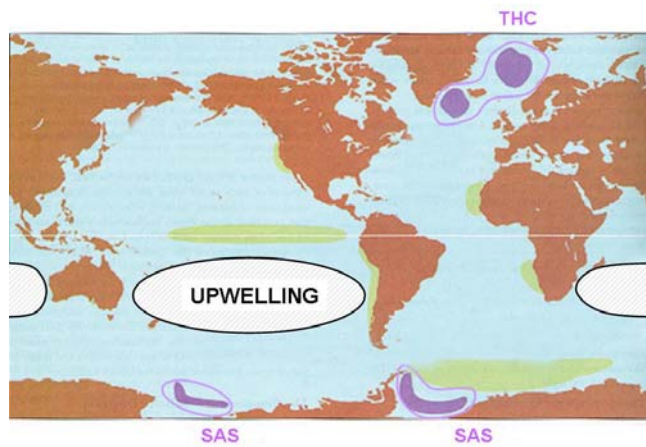
Figure 19. The MOC is thought to be a combination of the THC and SAS.
