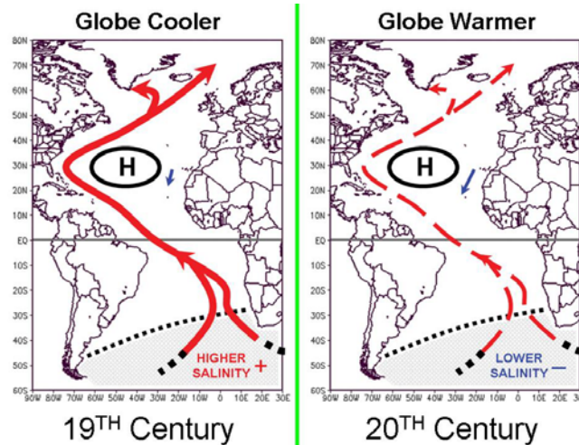
Figure 29. Idealized illustration of how the strength of the THC was likely stronger in the 19 th century than it has been through most of the 20 th century. These differences are hypothesized to be due to century-scale salinity variations.
