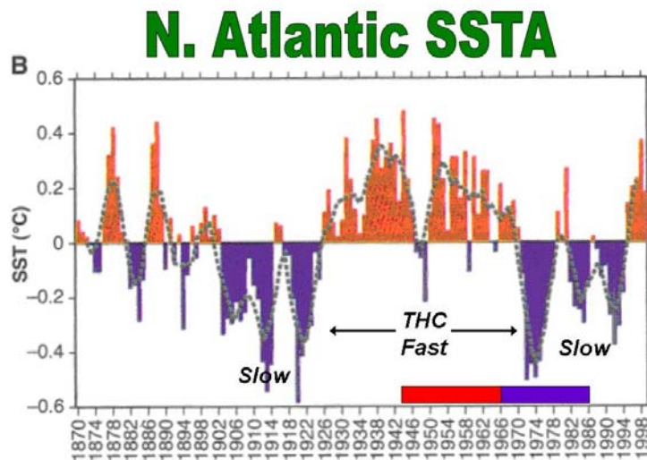
Figure 23. North Atlantic (50-65°N; 50-20°W) sea surface temperature anomalies (SSTA) from 1870-2000. Warmer temperature anomalies correspond to stronger than average THC conditions, and colder SST anomalies correspond to weaker than average THC conditions.
