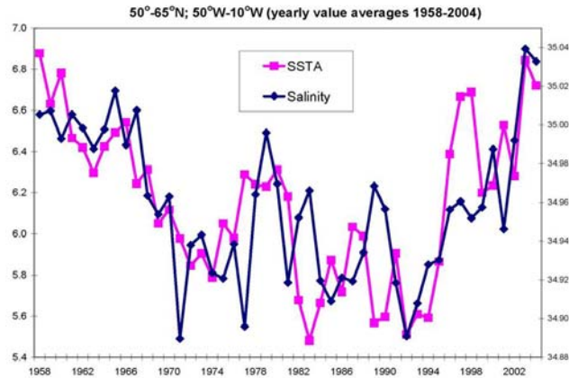
Figure 24. The close association between North Atlantic SSTA and observations of upper ocean salinity.
