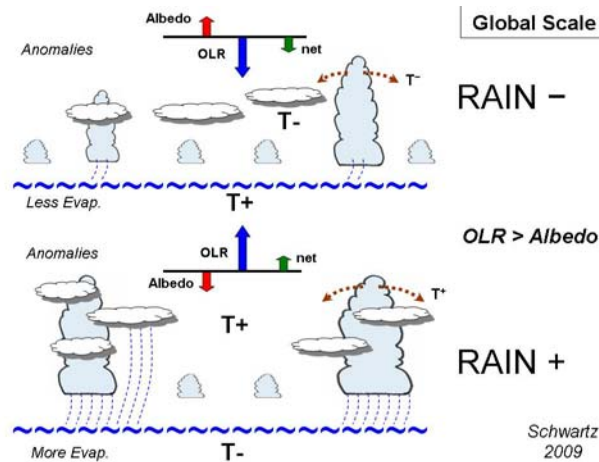
Figure 27. Idealized illustration of how the global troposphere maintains its neutral energy balance. When global surface evaporation and rainfall are suppressed (top), the troposphere receives less condensation warming and less radiation energy is sent to space. This causes the ocean to undergo warming. The opposite (bottom) occurs when there is enhanced surface evaporation and enhanced tropospheric condensation warming. More radiation energy is sent to space, and the greater surface evaporation causes upper ocean cooling.
