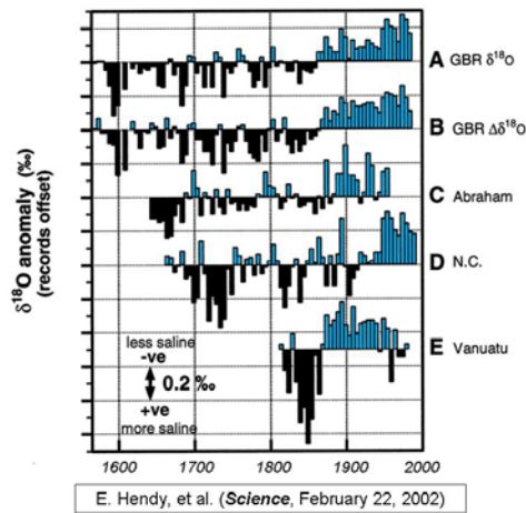
Figure 30. Inferred long period south Pacific salinity data indicating that 20 th century upper ocean salinity may indeed have been lower than in prior conditions.
