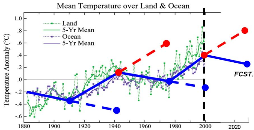
Figure 22. Illustration of how much error one would have made by extrapolating a cooling or warming curve beyond 30-35 years. The recent 1975-2000 warming trend should not be expected to continue. We have seen weak global cooling since 2001. I estimate global temperature by 2030 will be somewhat below the value of today's global temperature.
