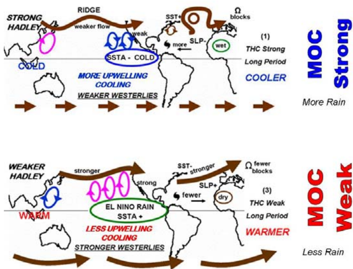
Figure 15. The top diagram shows the typical global wind patterns when the MOC has been strong for a long period and cold water upwelling in the Southern Hemisphere has been greater than the long period average. This leads to global temperatures becoming gradually cooler than average and more global rainfall (top diagram). The bottom diagram shows the typical global wind patterns when the MOC have been weaker than average for a long period and there has been reduced cold water upwelling in the Southern Hemisphere. The globe becomes gradually warmer during these periods and global rainfall is reduced. The top diagram shows characteristics of the conditions which existed during the modest global cooling period between the mid-1940s and the mid-1970s. The bottom diagram is characteristic of the conditions during the warming period of the mid-1970s to around 2000.
