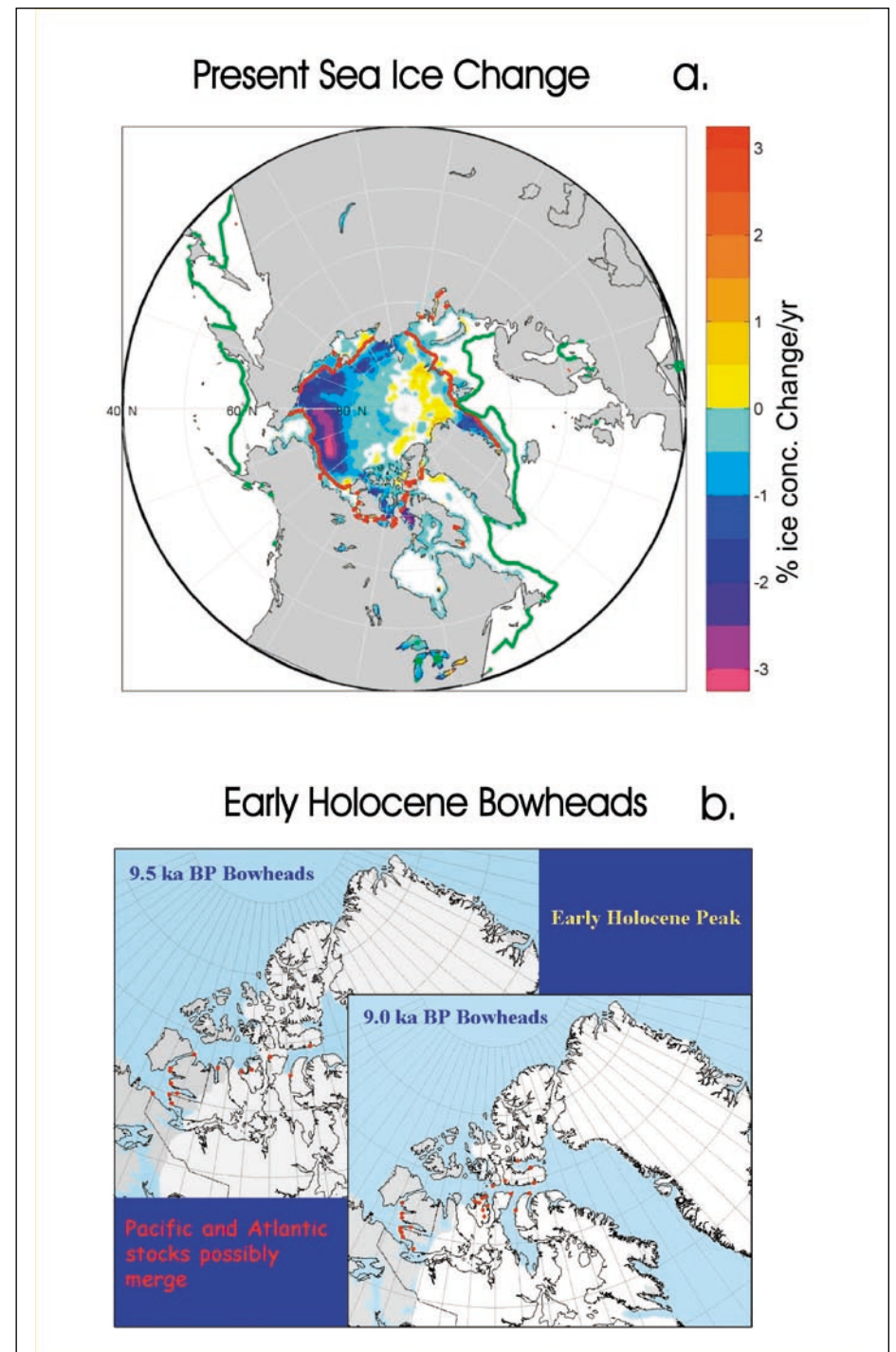
Fig. 1. (a) September ice trends and average minimum (September, red line) and maximum (March, green line) ice extents, 1979–2003 [Cavaliere et al. , 2004]. (b) Distribution of bowhead whale bones dated 9.5 \pm 0.25 and 9.0 \pm 0.25 ^{14}\text{C} kiloyears B.P. White areas are ice sheets.
