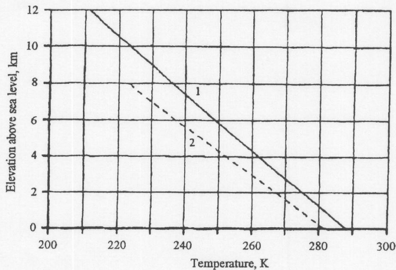
Figure 1. Relationship between the temperature and elevation above sea level for (1) existing nitrogen–oxygen atmosphere on Earth, and (2) hypothetical carbon dioxide atmosphere.
