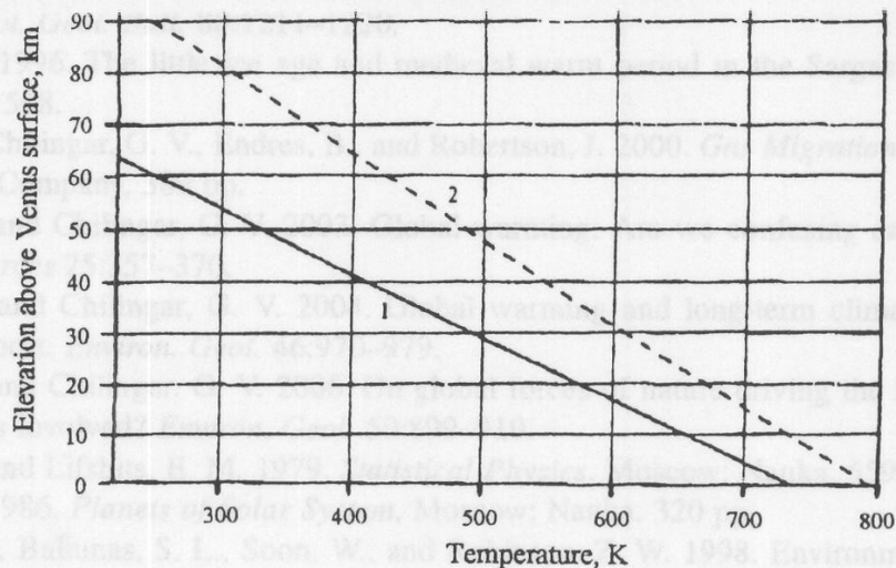
Figure 2. Relationship between temperature and elevation above Venus surface for (1) existing carbon dioxide atmosphere, and (2) hypothetical nitrogen–oxygen atmosphere.
