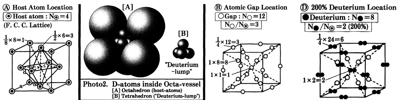
Figure 16. "Ultrahigh density metallic deuterium/hydrogen. The formation of condensed metallic deuterium lattice (hereafter, deuterium means deuterium/ hydrogen) (A) shows Pd fcc (face-centered cubic) lattice as a typical example of host metallic lattice. While (B) indicates the location of "atomic gap space" inside the host lattice. The location occupied with deuterium/hydrogen atoms corresponds to that of atomic gap space in (B) as seen (D)." "Photo2. Model of octahedral structure in unit cell of host lattice and the "deuterium lump" with ultrahigh density (simply "pynodeuterium-lump") which located with shape of tetrahedral structure inside the Octahedron of the host lattice. Here, this model is constructed using the ratio between actual Pd and deuterium in diameter."
