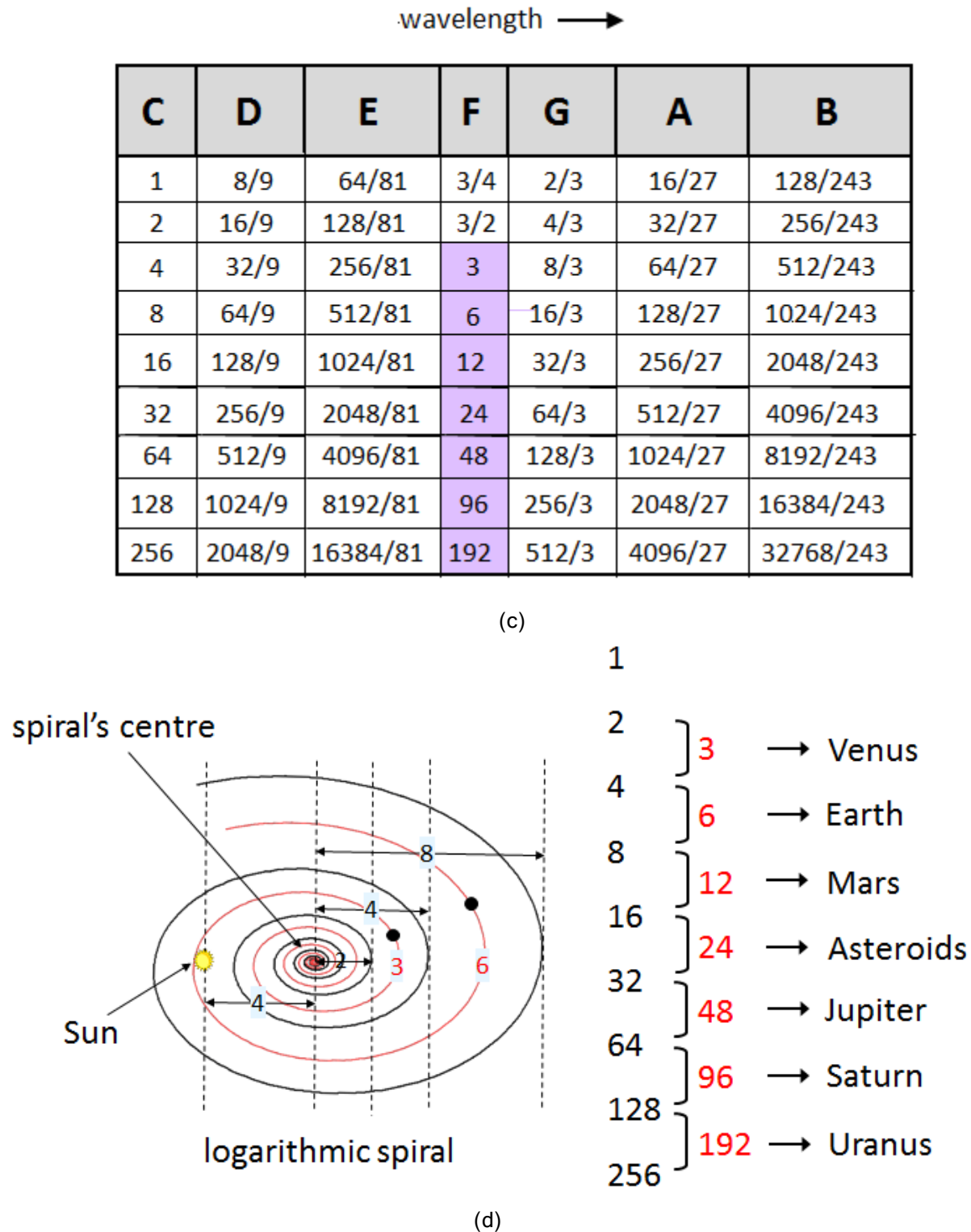
Figure 28 Spiral-cyclic analysis of our solar system. (a) the Pythagorean musical scale broken out into equal-tempered tones and semi-tones. The chart also shows the translation of colour into the musical tones. (b) shows the tone ratios of the seven octave species. Coloured cells denote notes of the Pythagorean (C) scale (notice that all its cells are coloured) and white cells denote non-Pythagorean notes. (c) the wavelengths of the undertones of the Pythagorean musical scale (d) Planetary mean distances from the spiral's asymptotic centre are perfect fourths of musical undertones of the F scale. (Phillips, 2010)
