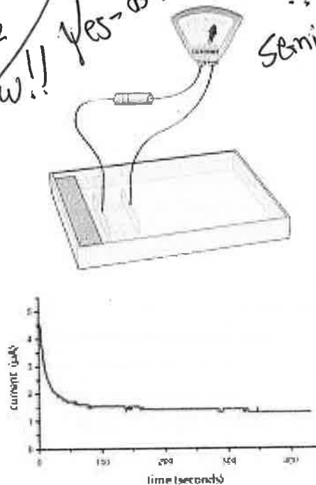
Fig. 5.6. Current flow from separated charges in EZ and the water beyond. Current begins flowing immediately after immersing electrodes, and maintains a non-zero plateau value for an extended period of time.
