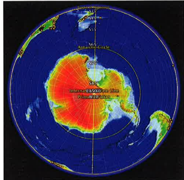
Fig. 1. Antarctica map distribution of petroglyphs. Upper left: South Australia and Tasmania. Upper center: New Zealand. Upper right: Easter Island. Lower right: Chile and Argentina. Lower left: South Africa. The yellow and red dots are GPS-logged petroglyph and pictograph sites, respectively. Brown denotes high altitudes while green denotes low altitudes.
