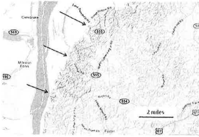
Fig 6. Eastern bank of the southern Mississippi River (34.967-87.083). Note evident floodplain that runs up to dendritic patterns in foothills. All dendritic patterns are completely self-affine, which is a trait not found in braided systems such as the Mississippi. However, such a characteristic is found in electrical discharges.
