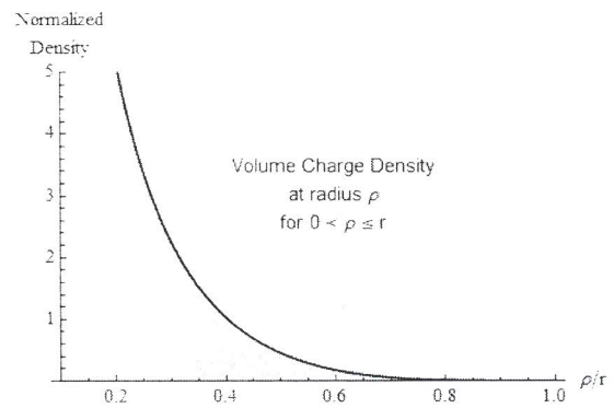
Figure 7. Normalized, Dimensionless Charge Density plotted as a function of \rho_r .
