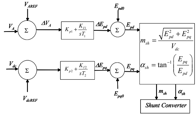
Figure 5. The UPFC shunt converter control.
