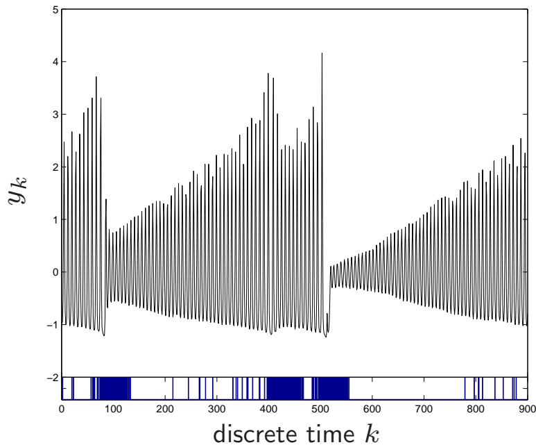
Santa Fe laser data
