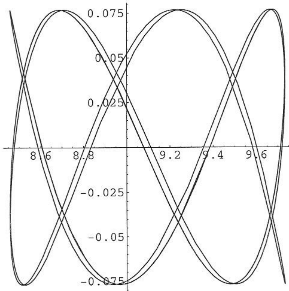
Fig. 3. The solar system's motion in the R-Z plane from 601 million years ago to 15 million years into the future.
