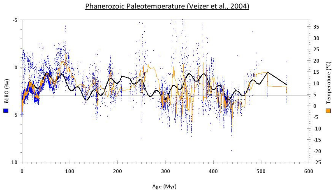
Fig. 5. Oxygen isotope paleotemperature data of the last 600 Myr compared with the solar system’s radial and vertical motion in the galaxy [6],[45] .
