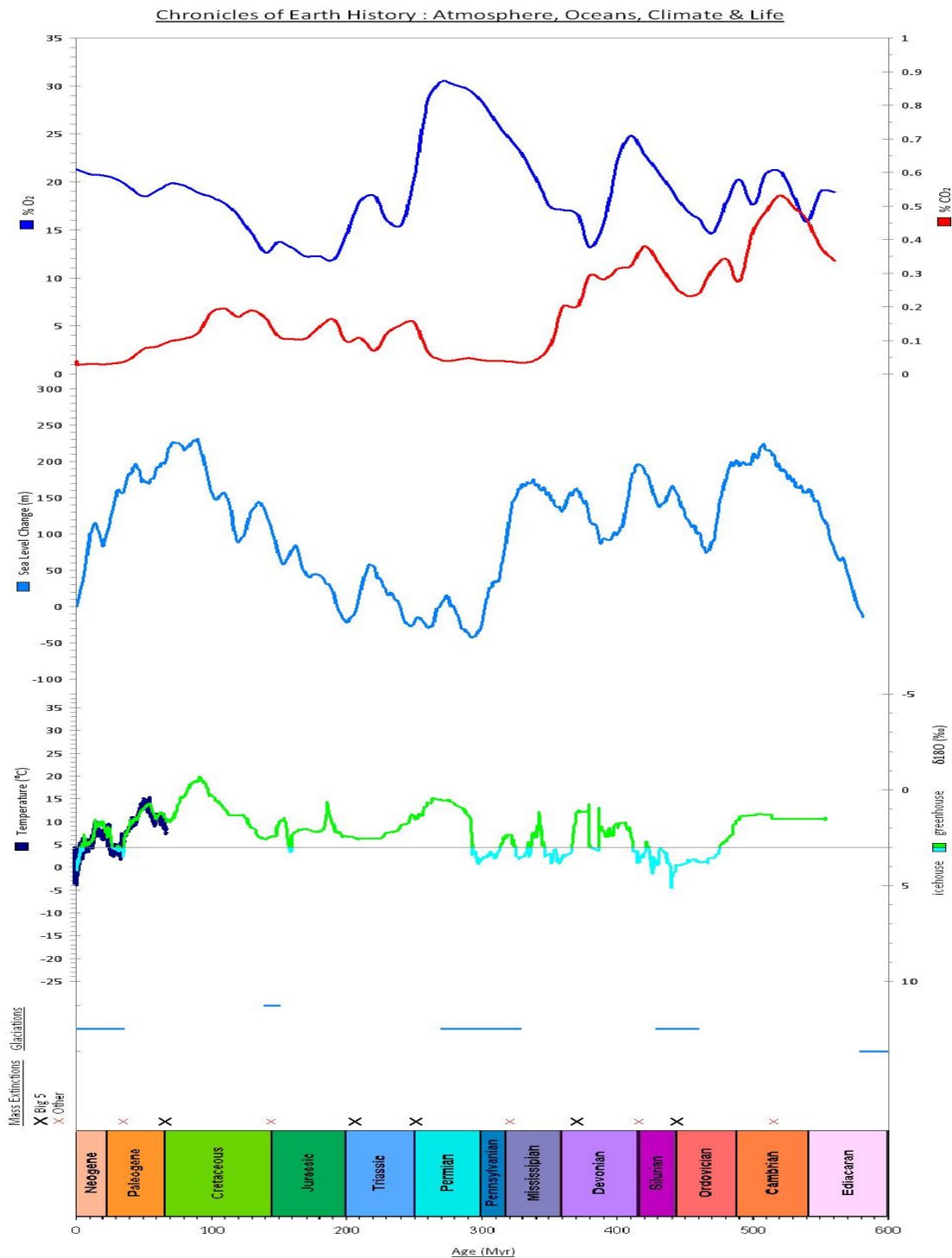
Fig. 1. Atmospheric concentration, sea level and temperature measurements and glaciations and extinction events over Phanerozoic time, based on the ICS Geological Timescale 2004 [35] .
