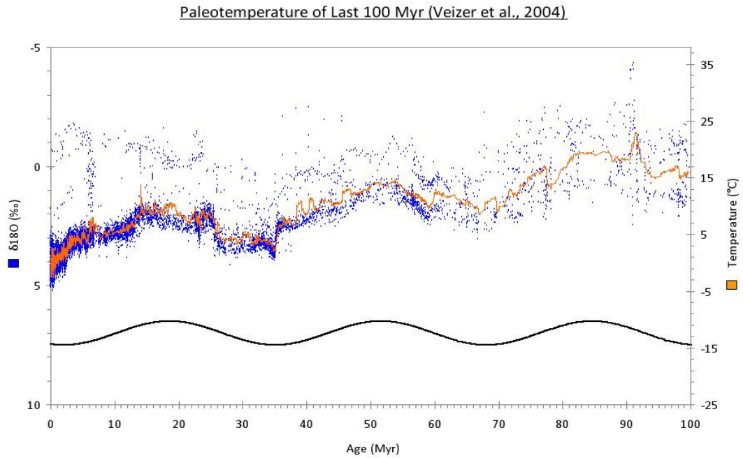
Fig. 4. Oxygen isotope paleotemperature data of the last 100 Myr compared with the solar system’s motion perpendicular to the galactic plane [6] .
