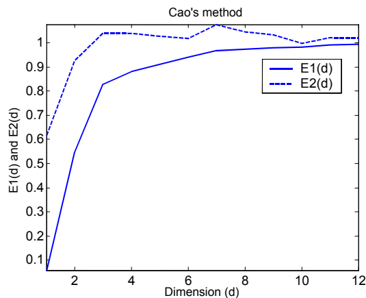
Fig. 6. Cao's method for the Yearly Sunspot Number.
