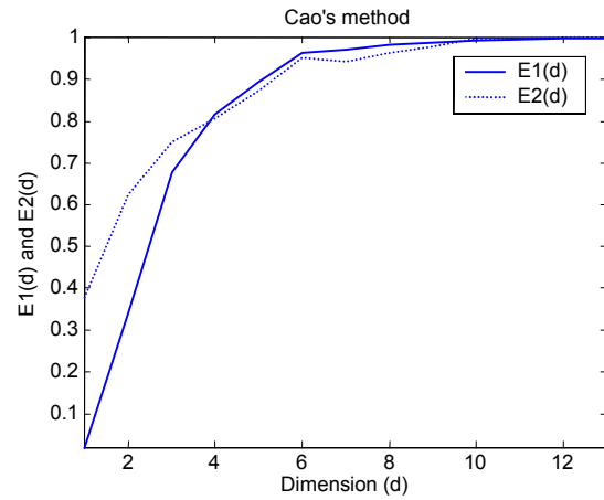
Fig. 10. Cao’s method for the R_{12} Index.
