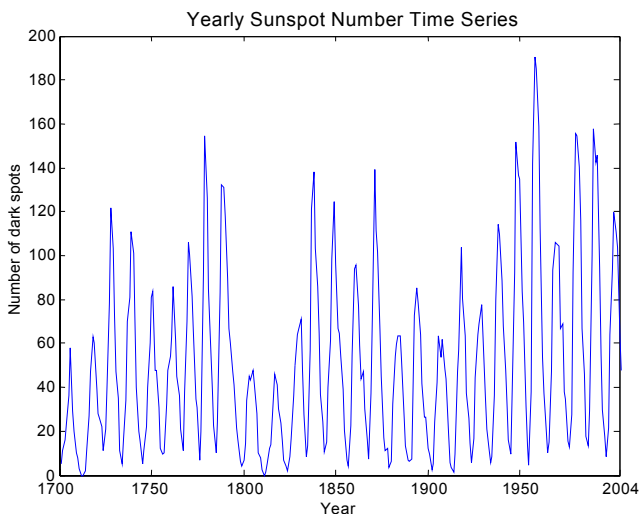
Fig. 2. Yearly Sunspot Number from 1700 to 2004.
