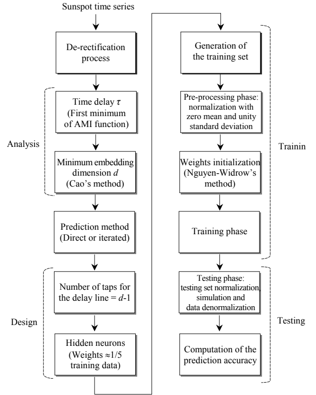
Fig. 5. Flow chart of the proposed methodology for sunspot data prediction.
