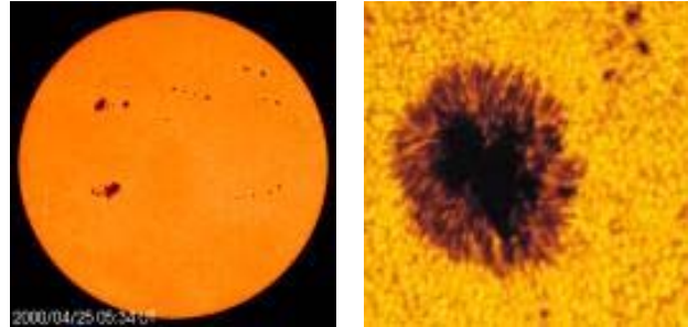
Fig. 1. Dark spots observed on the sun.
