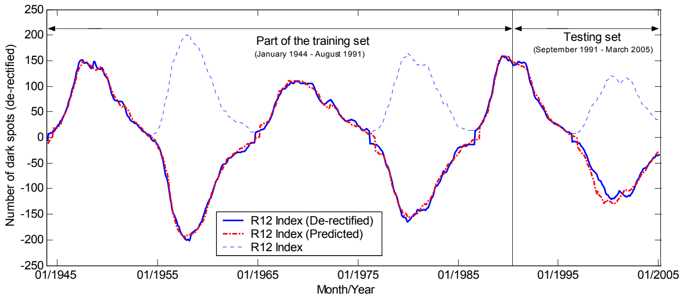
Fig. 11. 6-months ahead prediction of the R_{12} Index.
