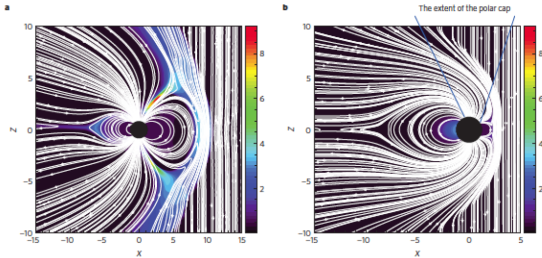
Figure 15. The magnetic field lines and plasma pressure in the Earth's magnetosphere due to a CME event. a , Initial state. b , Final state. Magnetic field lines (white) and plasma pressure in nPa (color map). Axes represent distance from the Earth's center in units of Earth radius (Airapetian et al. 2016).
