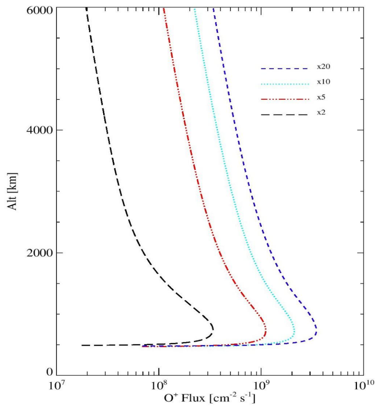
Figure 14. The mass loss rate of oxygen ions from the Earth atmosphere due to XUV flux from the young Sun at F_{XUV}=2 F_0 (long dash), 5 F_0 (dash-dot), 10 F_0 (dot), 20 F_0 (short dash) (from Airapetian et al. 2017a).
